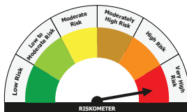
Scheme Riskometer
