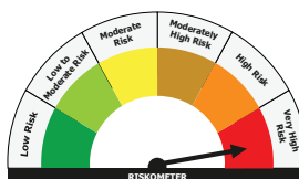
Scheme Riskometer
